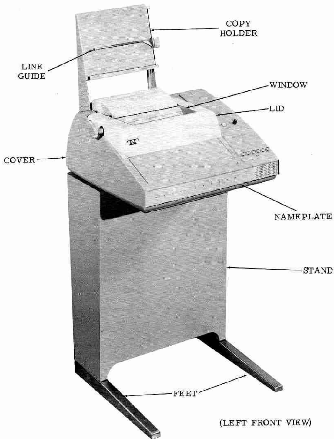
Figure 2 — Receive-Only (RO) Teletypewriter Set
