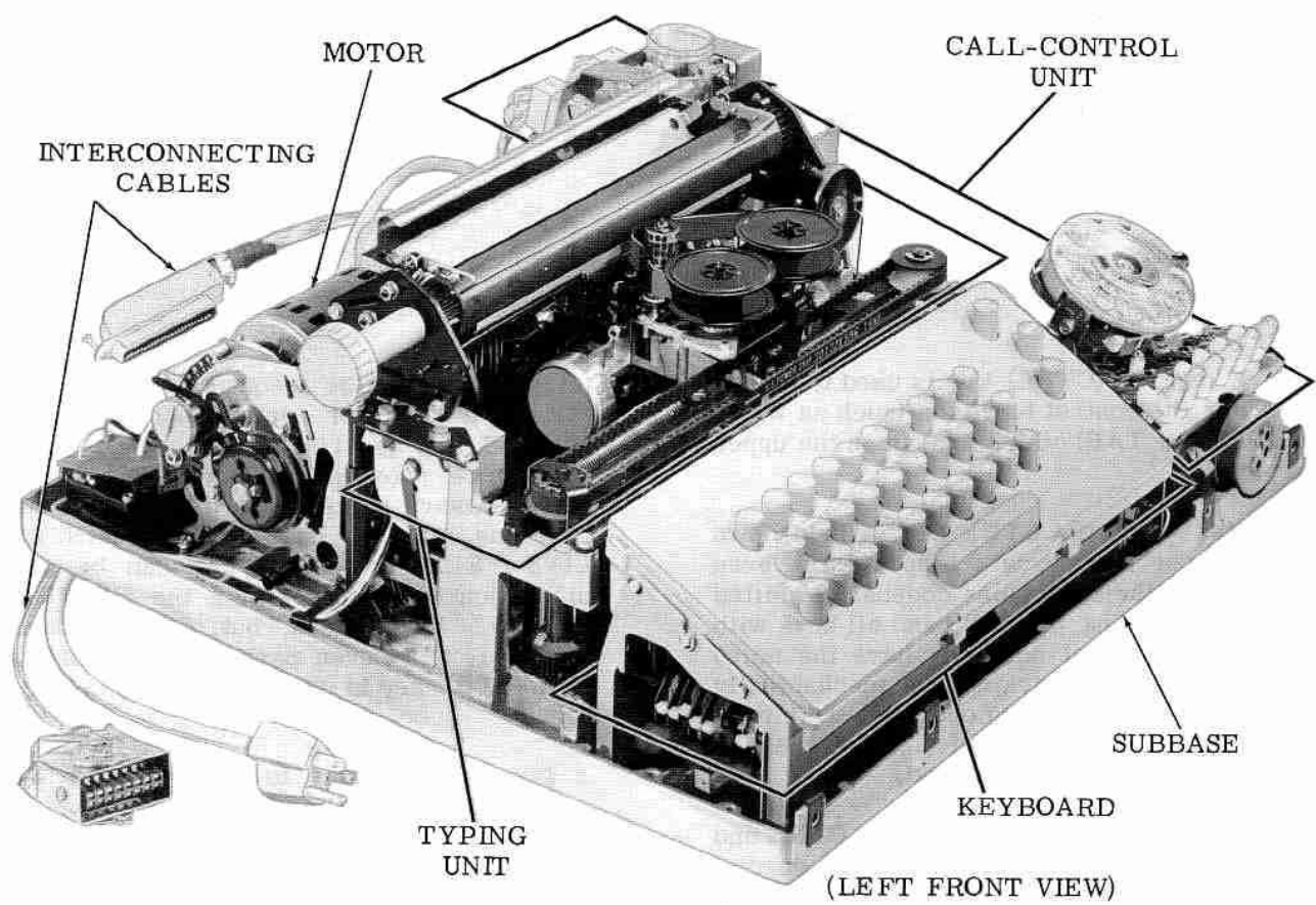
Figure 5 — Keyboard Send-Receive (KSR) Teletypewriter Set (Without Cover)
