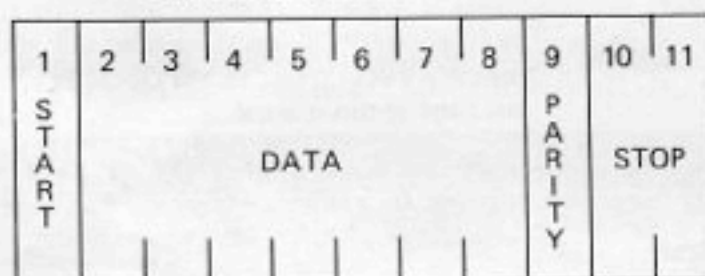
Bit Structure of Serial Data Word
