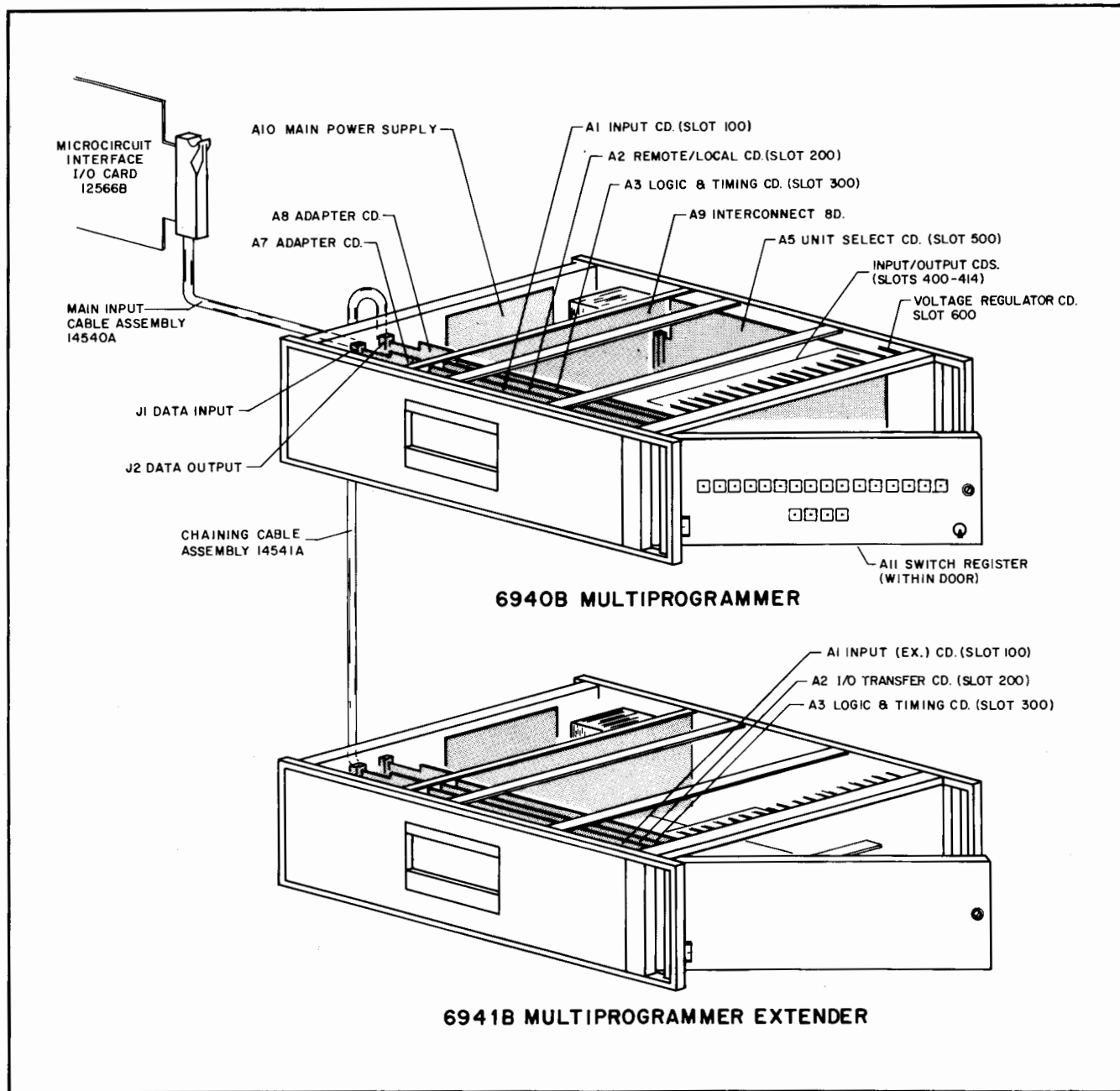
Figure 1-1. System Configuration
