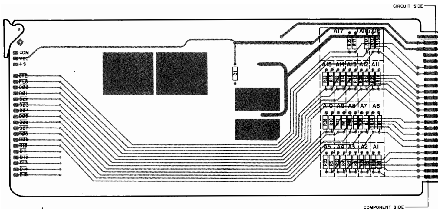
A1 Standard Input Card, Component Locations
