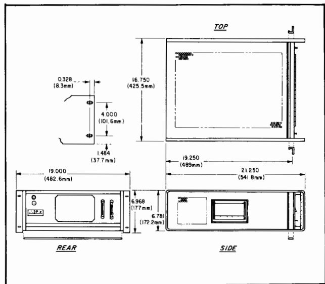
Figure 2-1. Outline Diagram
