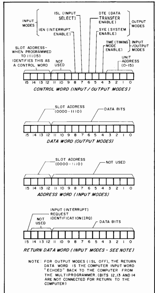
Figure 3-6. Word Formats
