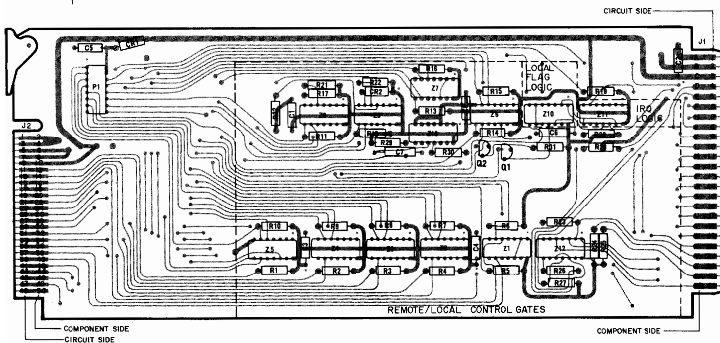
A2 Remote/Local Card, Component Locations
