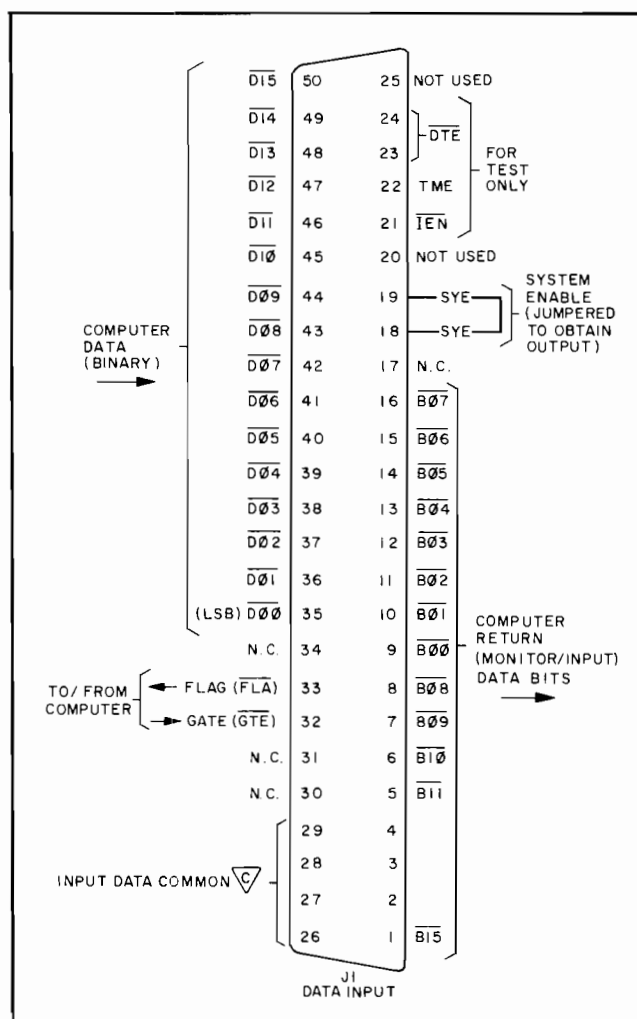
Figure 3-1. Data Input Connector
