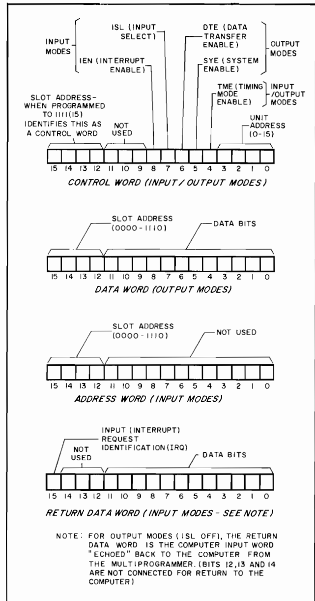
Figure 3-6. Word Formats
