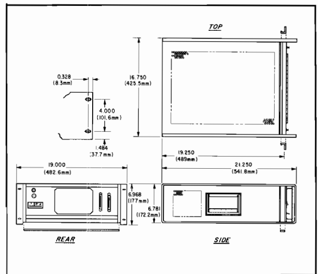
Figure 2-1. Outline Diagram
