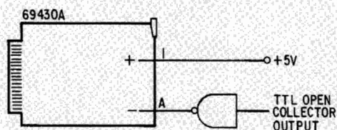
SUGGESTED CONFIGURATION TO DRIVE THE 69430A INPUTS WITH TTL SIGNALS
