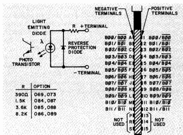
SUGGESTED CONFIGURATION TO DRIVE THE 69430A INPUTS WITH TTL SIGNALS
