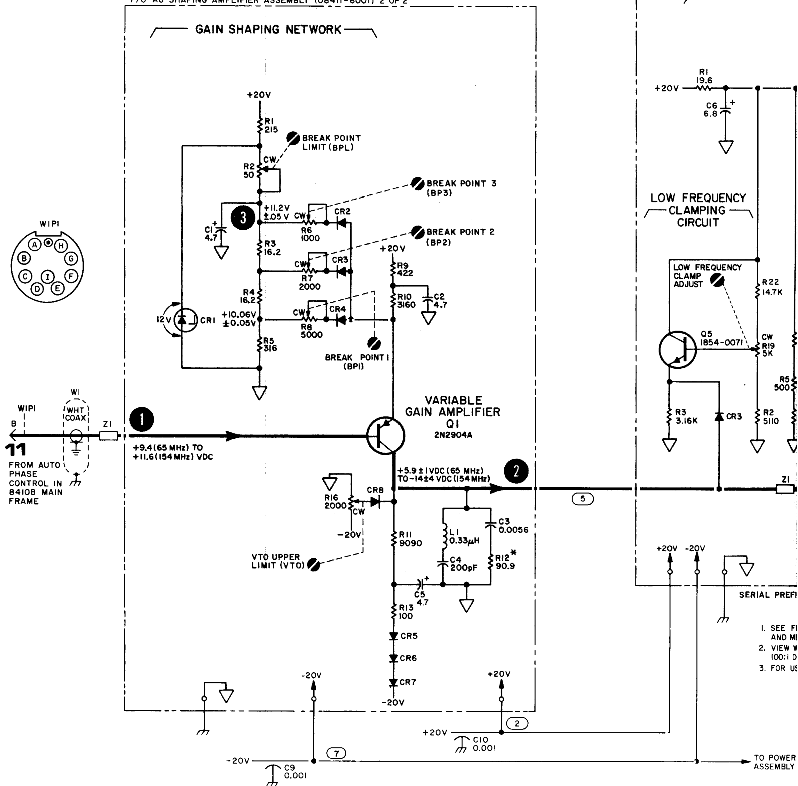
P/O A6 SHAPING AMPLIFIER ASSEMBLY (08411-6001) 2 OF 2
