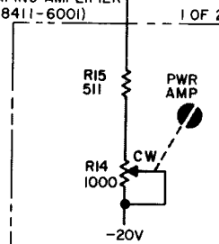
Figure 8-27. 8411A-A1, A2, A3, and Stripline Schematic Diagram
