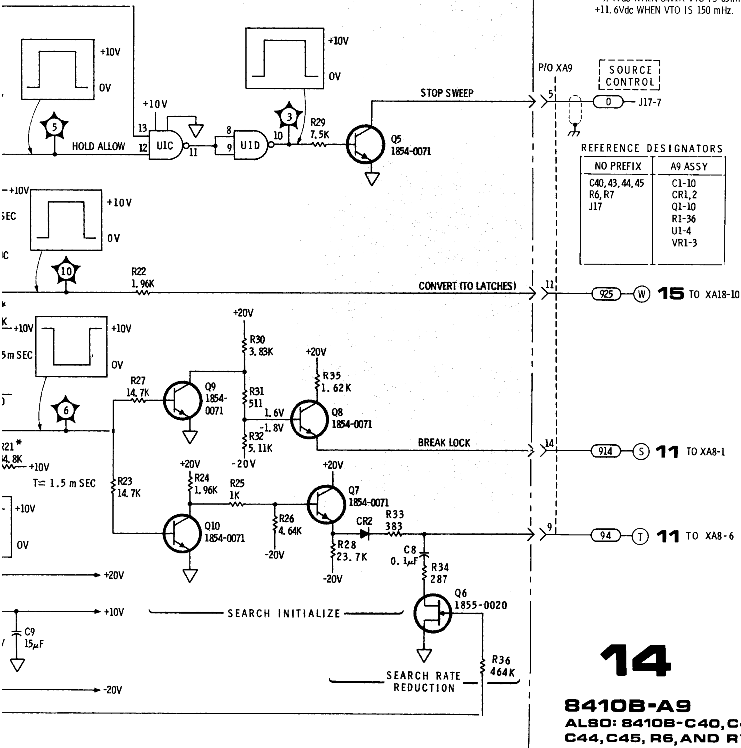
Figure 8-64. 8410B-A9 Schematic Diagram
