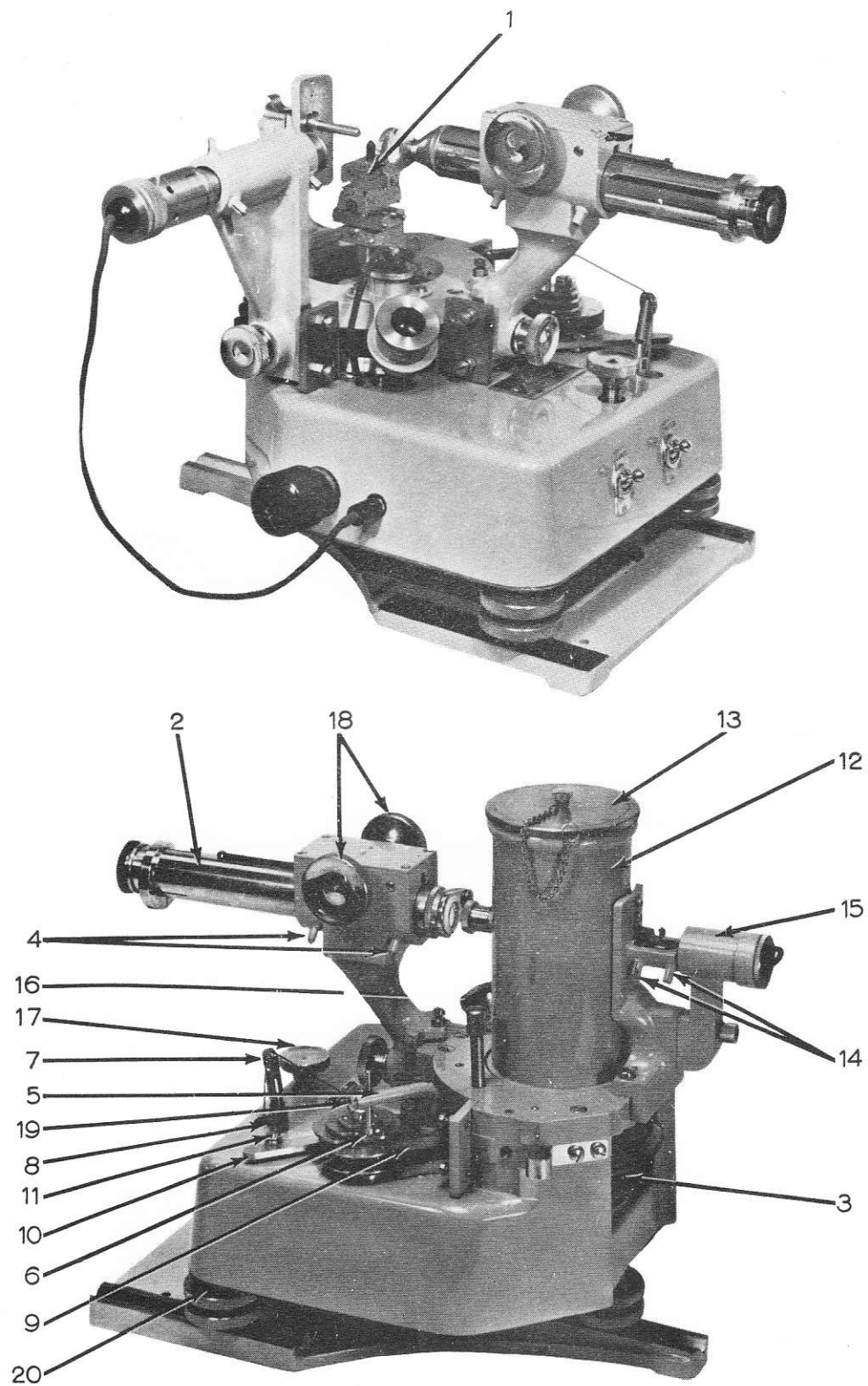
Fig.1 S.25 Single Crystal Goniometer
