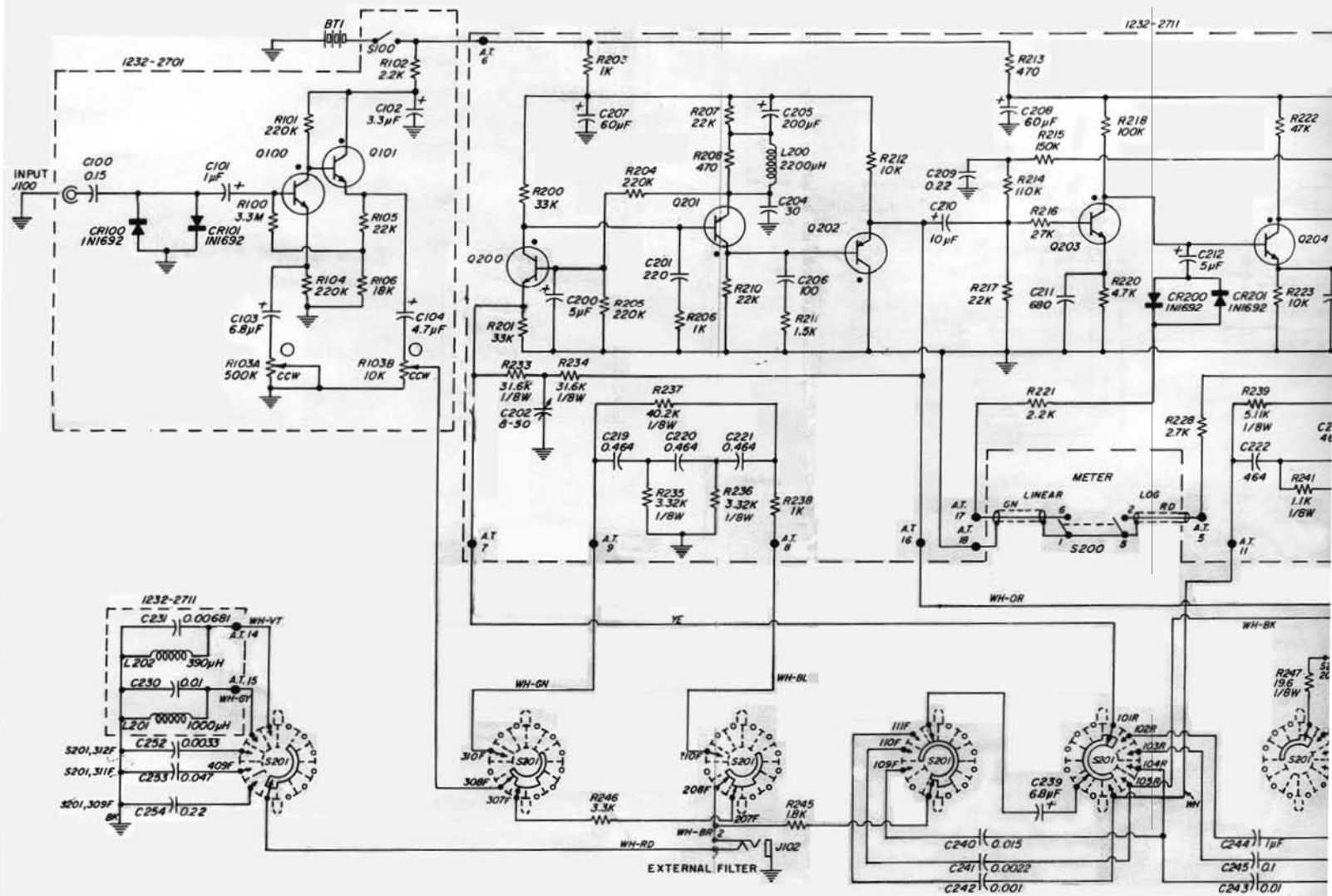
Figure 8. Schematic diagram of the Type 1232-A Tuned Amplifier an
