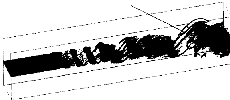
Fig. 5. – Run NFSQ2D; isosurface \|\omega\| = 2/3\omega_i .
