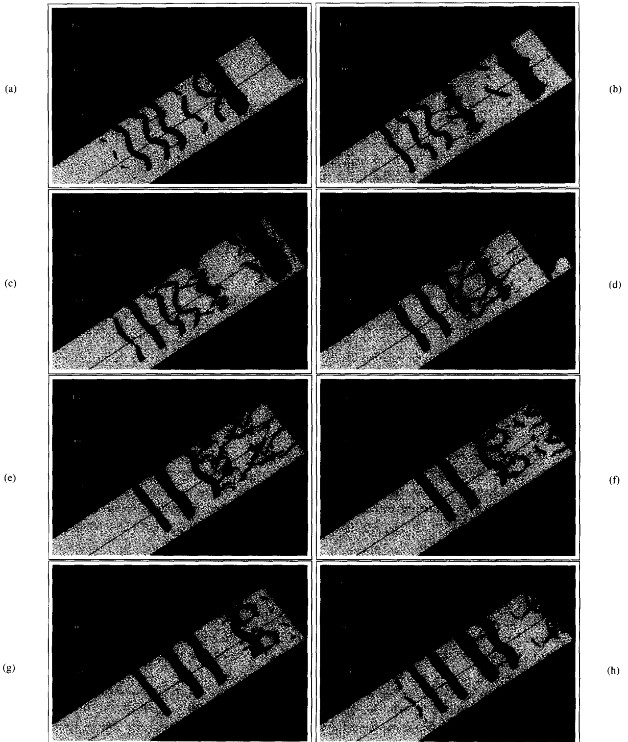
Plate 1. – Time evolution of the most intense vortices (run NFSQ2D, domain duplicated in spanwise direction). Isosurfaces \langle p(t) \rangle - p_{rms}(t) coloured by \omega_{3D} = (\omega_x/|\omega_x|) \cdot \sqrt{\omega_x^2 + \omega_y^2} . Zero corresponds to green, values larger than 0.6 \omega_i to red and values smaller than -0.6 \omega_i to blue.
