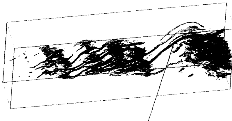
Fig. 6. – Run FSQ2D; iso-surfaces \omega_x = 0.5\omega_i (black) and \omega_x = -0.5\omega_i (light grey). Portion x < 40\delta_i of domain not shown.
