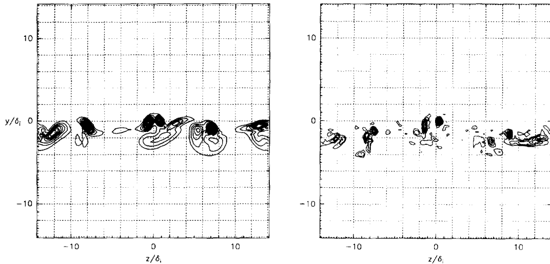
Fig. 2. – Cross-section of the vorticity magnitude showing cuts of longitudinal vortices, with full resolution on the left (DNS at Re = 100 ), and in LES at Re \geq 2000 on the right, in fully de-aliased pseudo-spectral simulations at resolution 96^3 .
