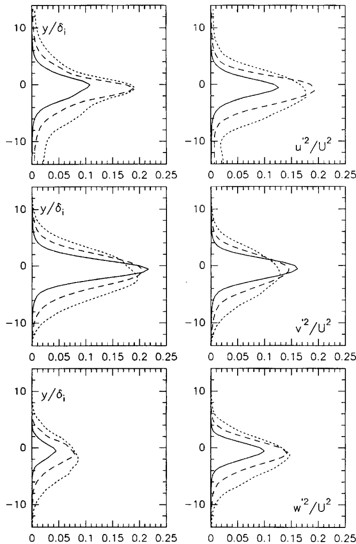
Fig. 12. – Profiles of the variance of the velocity fluctuations in run NFSFQ2D (left) and WFSF3D (right) at x = 58 \delta_i (—), x = 81 \delta_i (- -) and x = 104 \delta_i (...).
