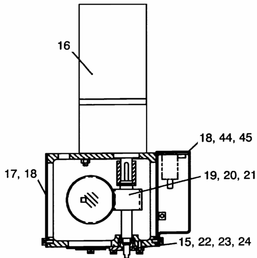
WORM GEAR & PINION ARRANGEMENT
