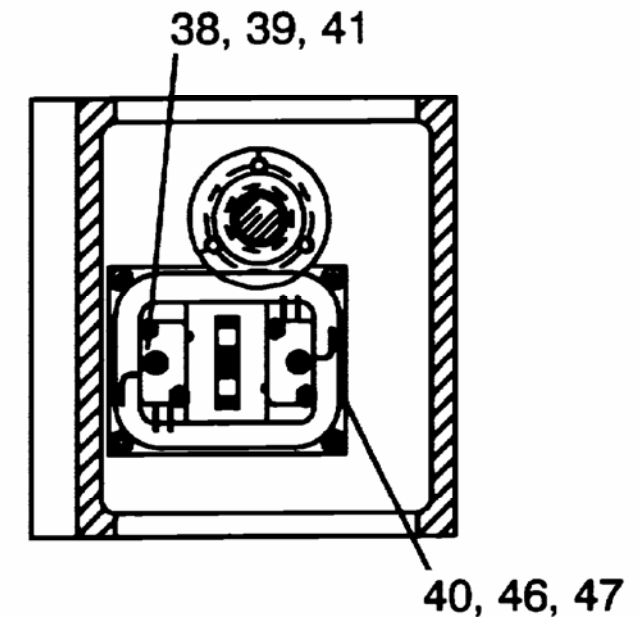
SECTION A-A LIMIT SWITCH ASSEMBLY STYLE I
