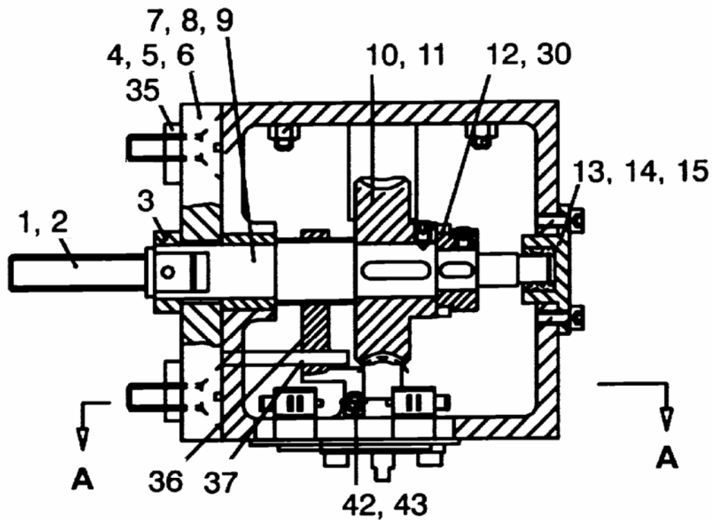
MOTOR DRIVE HOUSING ARRANGEMENT WITH STYLE I LIMIT SWITCH
