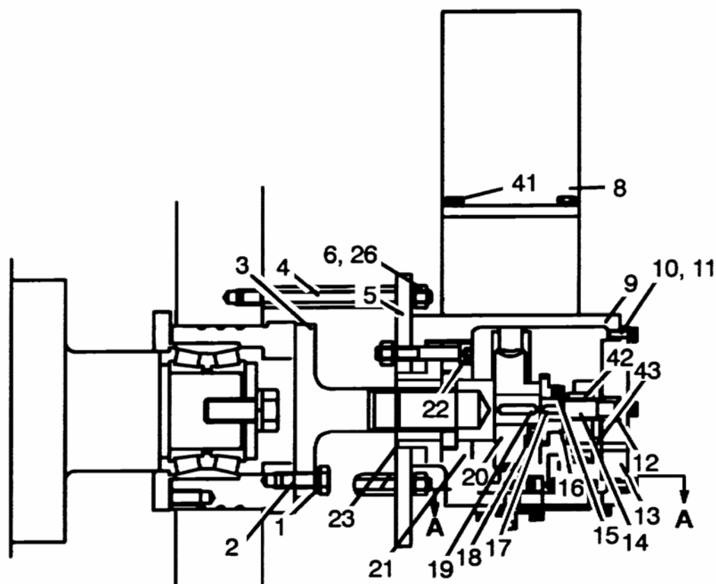
MOTOR DRIVE HOUSING ARRANGEMENT WITH STYLE I LIMIT SWITCH
