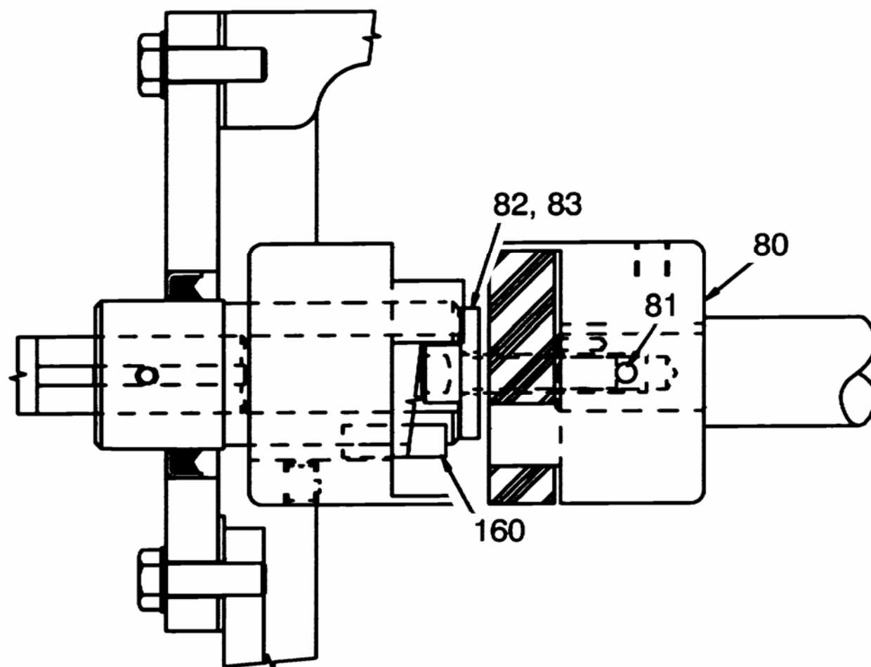
DETAIL "B"
