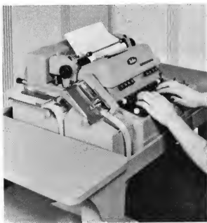
Flexowriter edge punches cards manually or automatically from punched paper tape.
