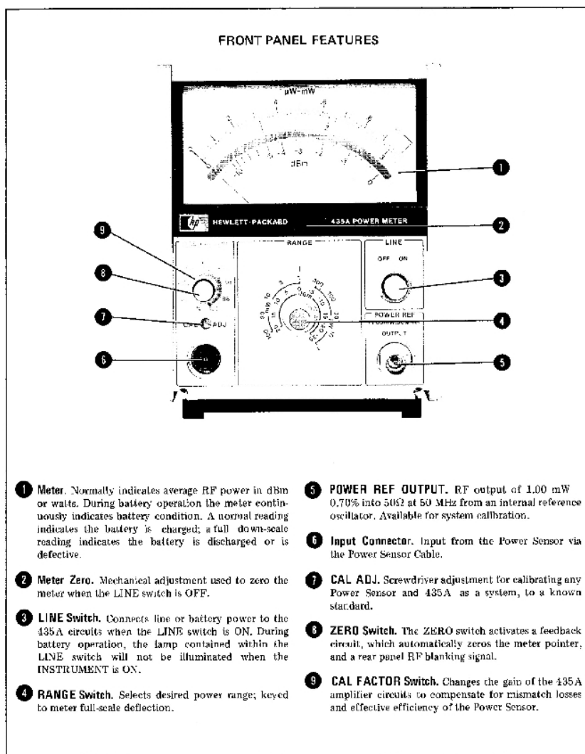
Figure 3-2. Front Panel Controls, Connectors, and Indicators
