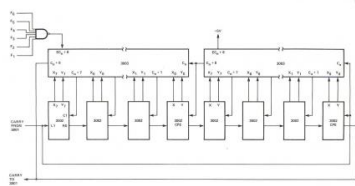
Figure 3. Carry Look-Ahead Configuration with No Carry Ripple through the Left Slice (32 Bit Array)
