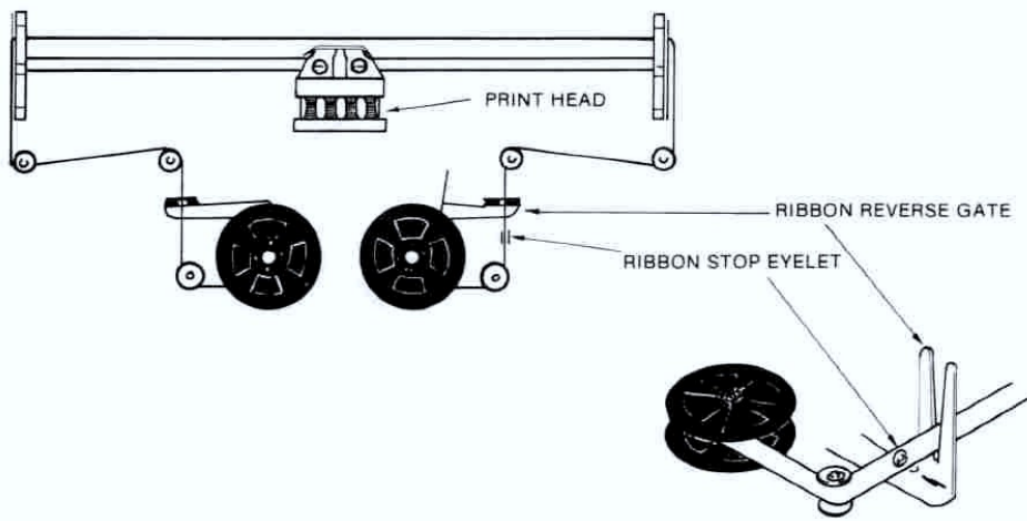
Figure 3. The Printer Ribbon Path
