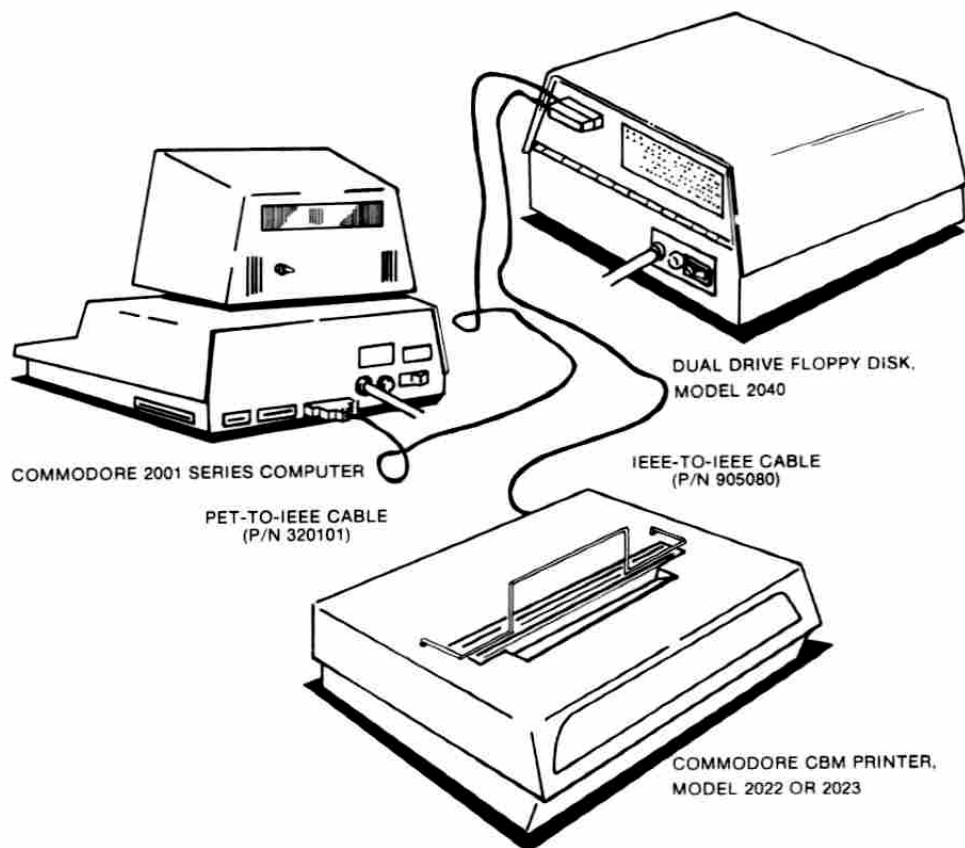
Figure 5. Multiple Hookup
