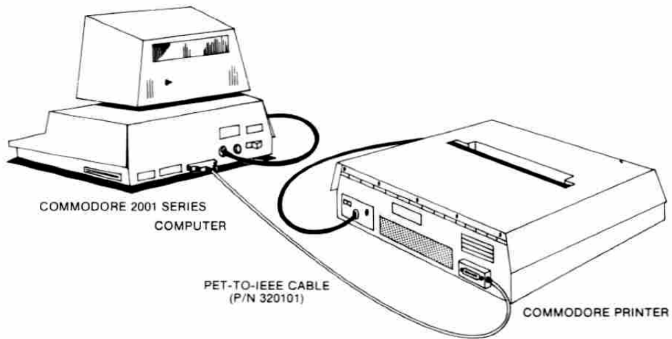
Figure 4. Printer to Computer Hookup
