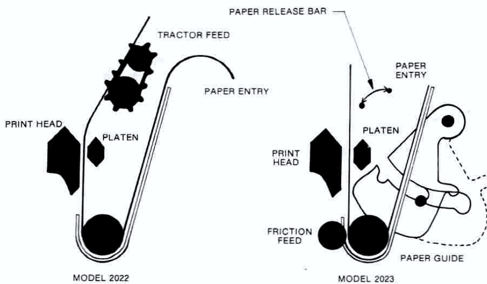
Figure 6. Paper Paths
