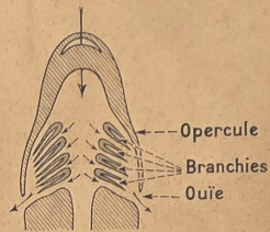
APPAREIL BRANCHIAL
