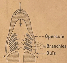
APPAREIL BRANCHIAL
